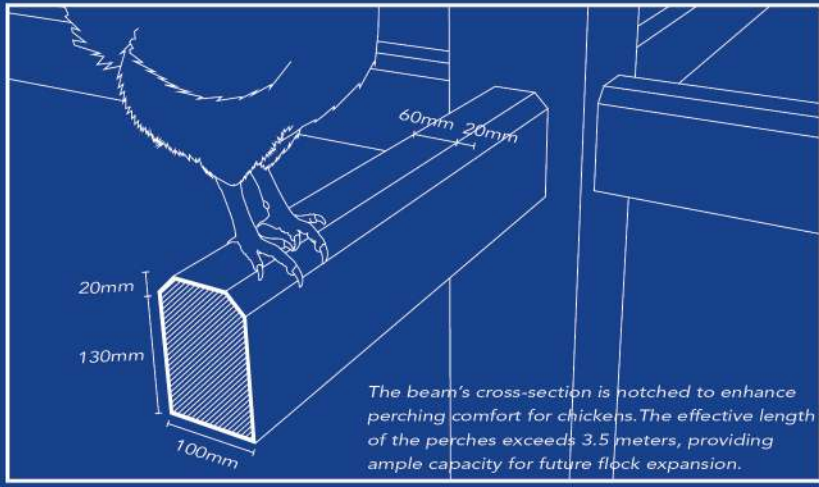
Perche ( beam )
