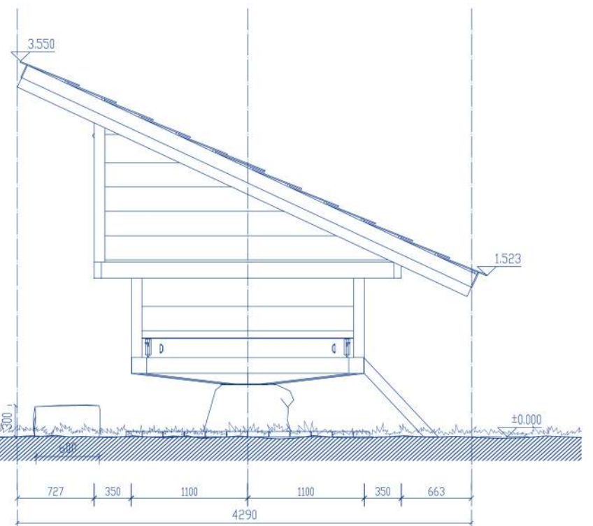
South & North Elevation 1:50
