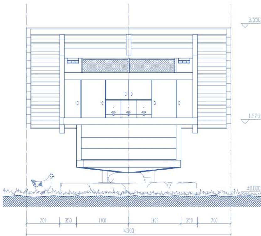
East Elevation 1:50
