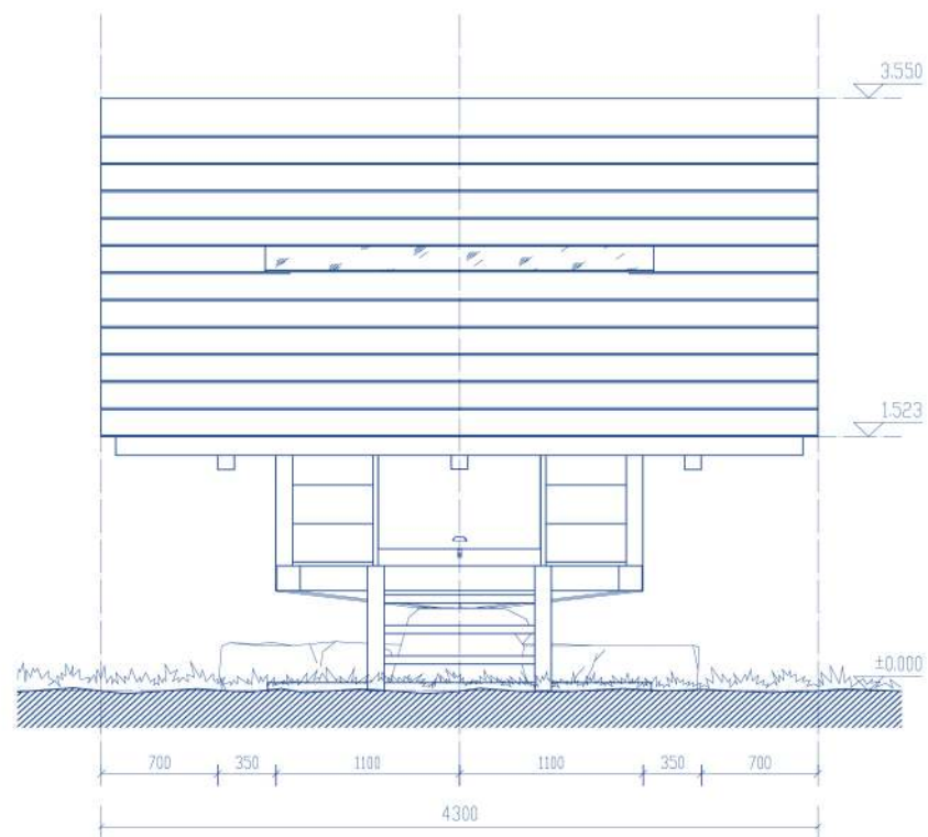
West Elevation 1:50
