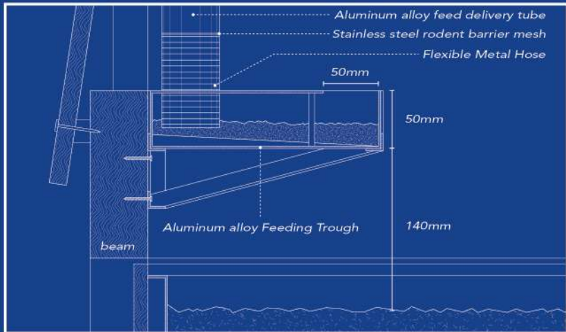
Feeding Trough
